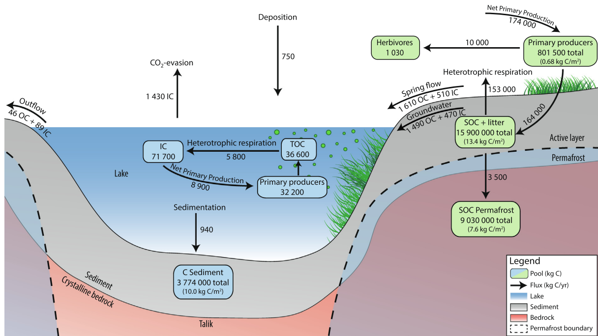
Fig. 5. Conceptual illustration of the carbon landscape ecosystem model for the TBL catchment with pools (kg C) and fluxes (kg C yr -1 ). Values per unit area are calculated using the area of the entire terrestrial or aquatic system.
